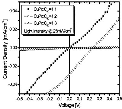
그림 3. Current density-voltage characteristics of ITO/CuPc/C 60 /Al device depending on thickness ratio of CuPc/C 60 heterojunction under 25mW/cm 2 .
