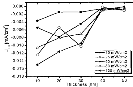
(b) short-circuit current density-thickness.
