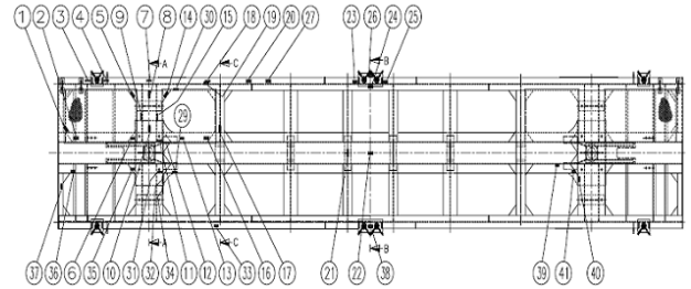
Fig. 1 Setting drawing of strain gauge
