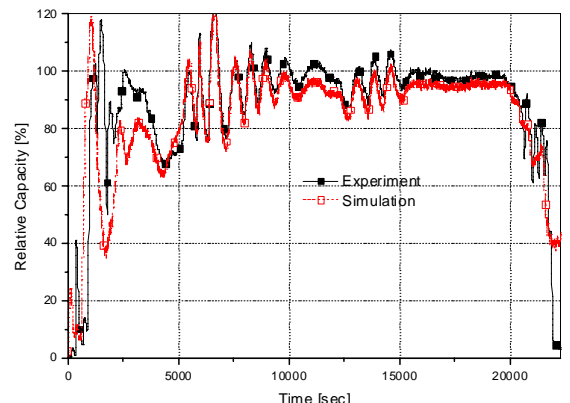
(g) Relative Cooling Capacity
