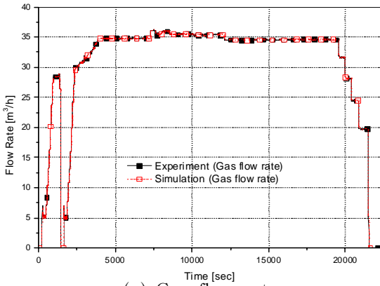
(a) Gas flow rate
