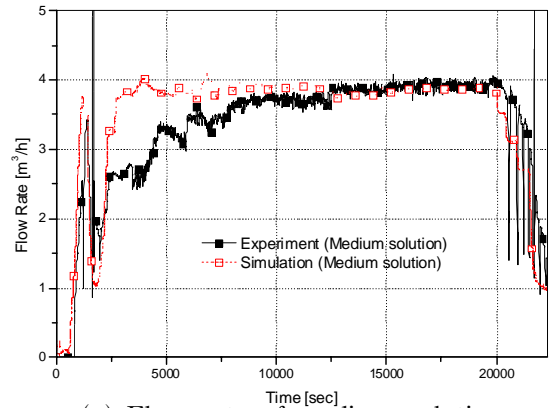
(e) Flow rate of medium solution
