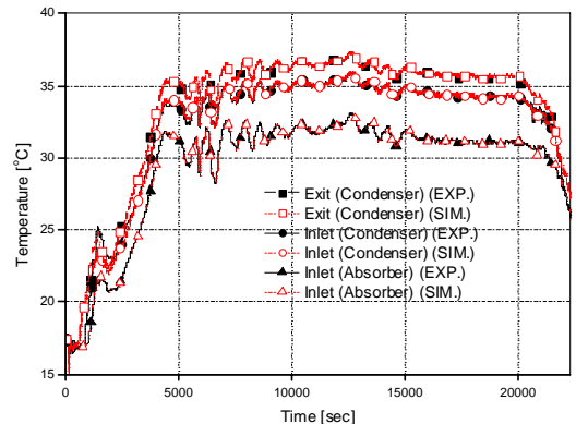
(a) Cooling water temperatures
