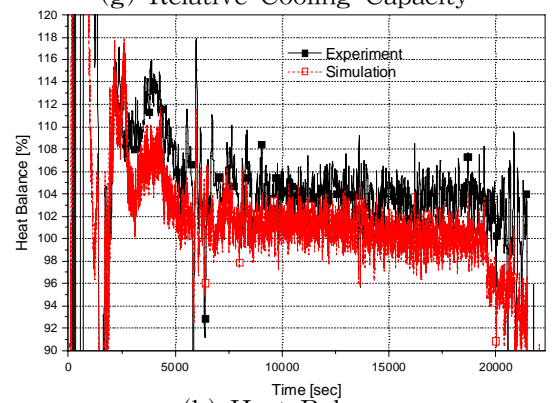
(h) Heat Balance
