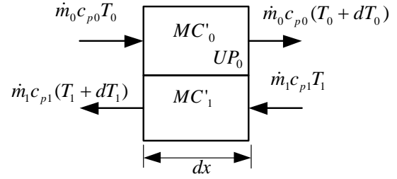
Fig. 2 Notation for heat transfer at an arbitrary segment surface of the model of a counter-flow heat
