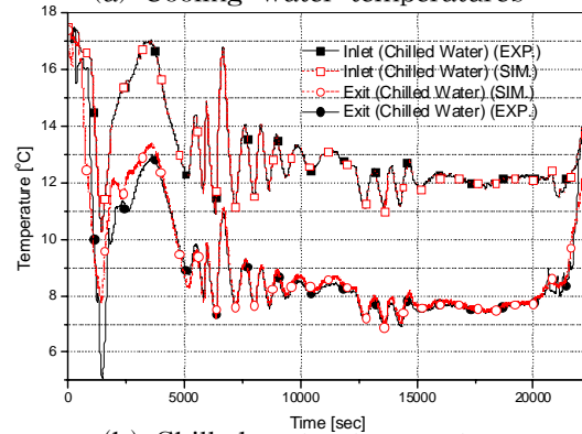
(b) Chilled water temperatures
