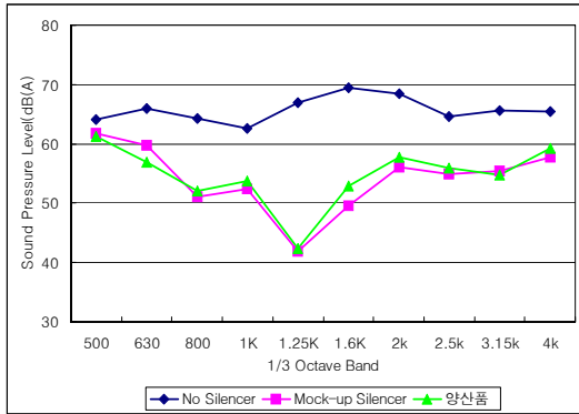
Fig.11 Noise reduction data of mass-produce silencer
