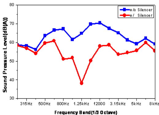
Fig.9 Noise reduction data of mock up silencer
