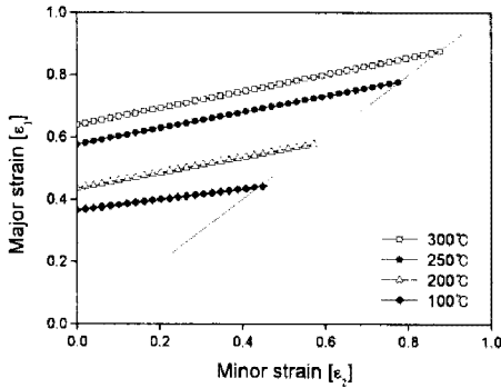
Fig. 8 FLCs at various temperatures
