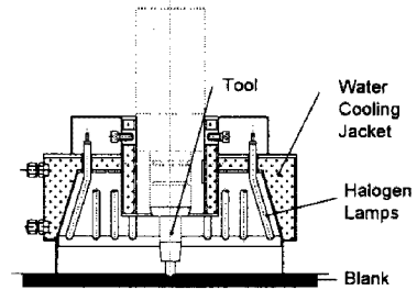
Fig. 3 Schematic of heating device
