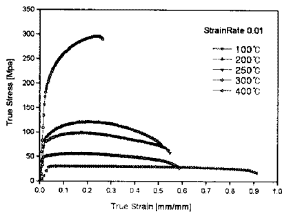
Fig. 1 Flow stresses at various temperatures and strain rates
