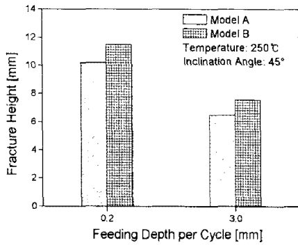
Fig. 4 Effect of process parameters: Feeding depth
