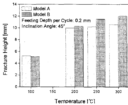
Fig. 5 Effect of process parameters: Forming temperature
