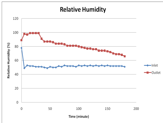
Figure 4. Relative Humidity Inlet and Outlet
