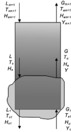
Figure 2. Continuous counter flow adiabatic packed column
