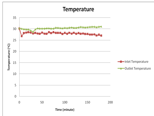
Figure 5. Temperature Inlet and Outlet
