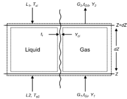
Figure 3. Differential section of a packed column
