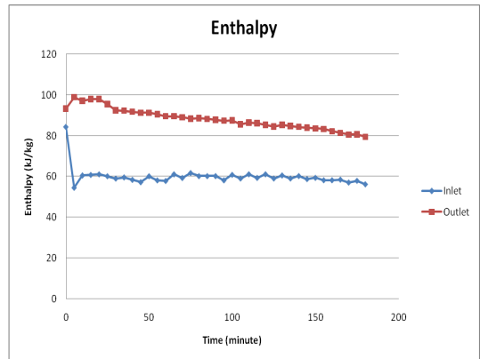
Figure 6. Enthalpy Inlet and Outlet
