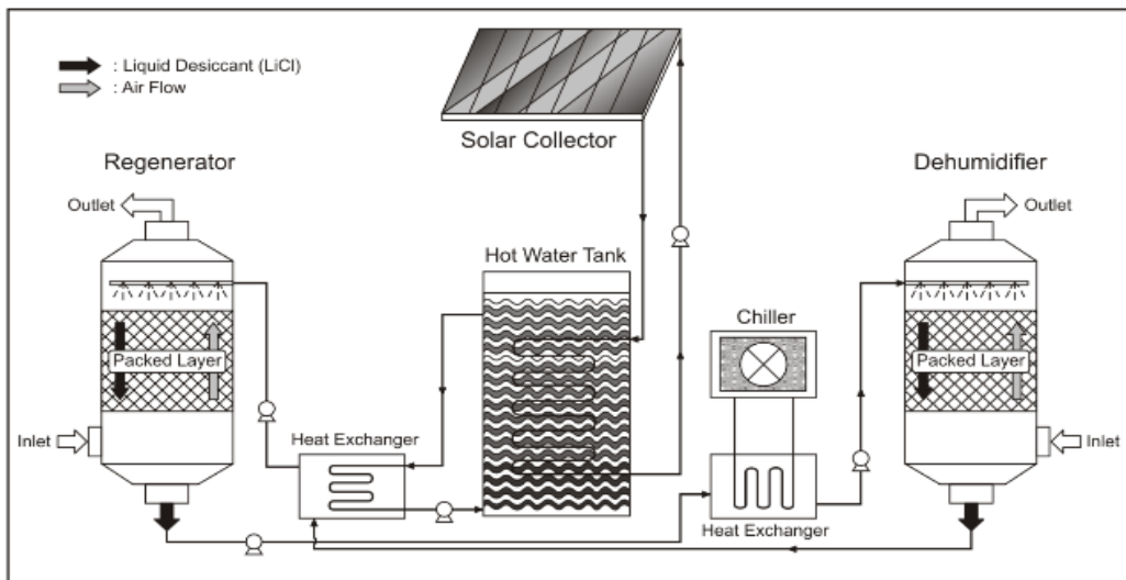
Figure 1. The Regenerator and Dehumidification System
