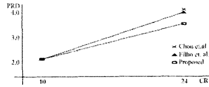
Fig. 5. Performance comparison among various ECG compression schemes record 100.
