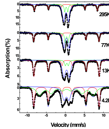
Fig. 2. The Mössbauer spectra of \text{Sn}_{0.97}\text{Fe}_{0.03}\text{O}_2 at various temperatures.
