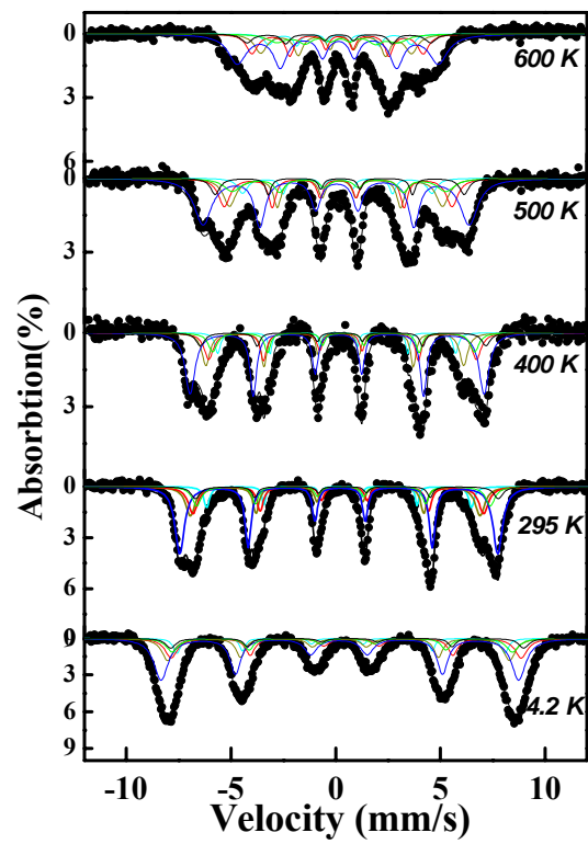
Fig. 1 Mössbauer spectra of \text{Ba}_2\text{Co}_2\text{Fe}_{12}\text{O}_{22} at various temperatures.
