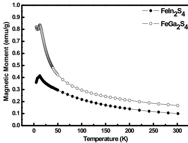
Fig. 1. The zero field cooled (ZFC) magnetic moment under B = 5000 Oe for \text{FeIn}_2\text{S}_4 and \text{FeGa}_2\text{S}_4 .
