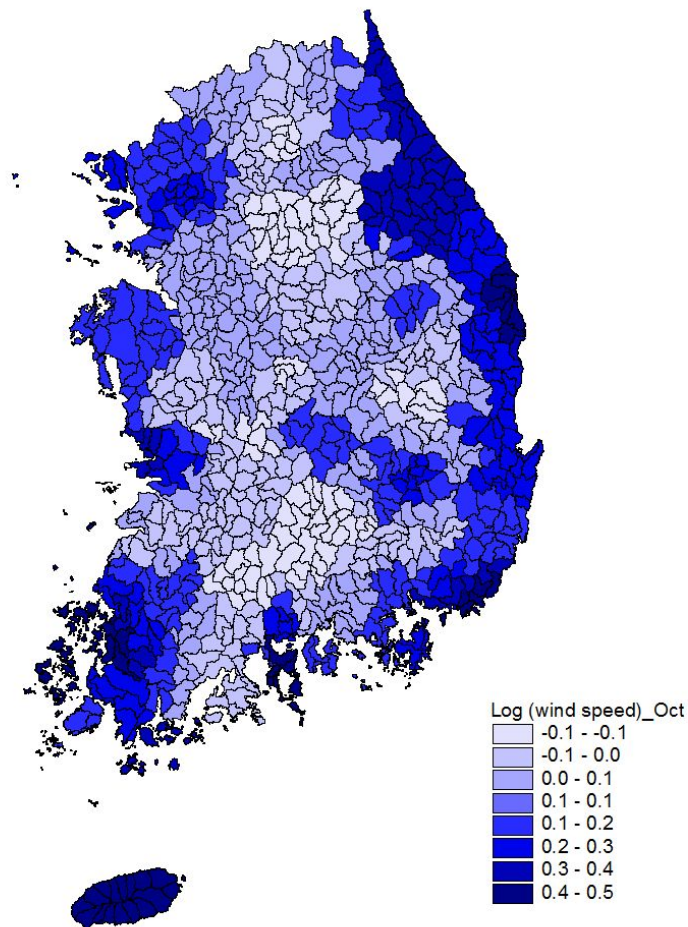
Fig. 2. The distribution of log transformed mean wind speed by catchment unit (October).
