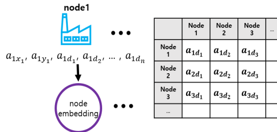
(b) GVRP
