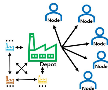
(a) VRP
