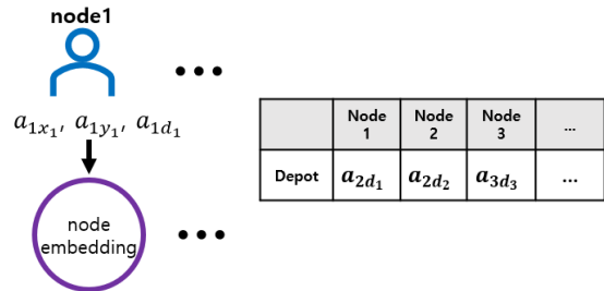
(a) VRP
