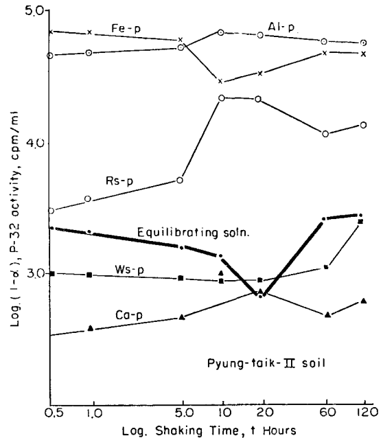
Fig. 13. Relationship between log. (1-α) of Ws-P, Al-P, Fe-P, Rs-P, Ca-P fractions and Equilibrating solution and log. t, the various reaction time, obtained from the Edgington Equation (from Shim, 1971)
