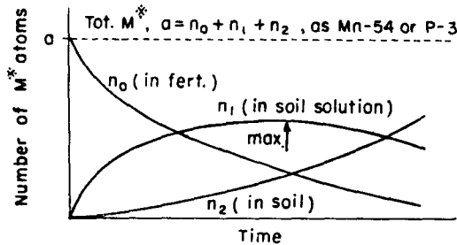
Fig. 4. Diagram showing the number of M* atoms, n, in the phases 0, 1, or 2 as a function of time.
