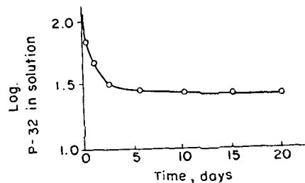
Fig. 3. Rate of isotopic dilution (Russell et al, 1961)
