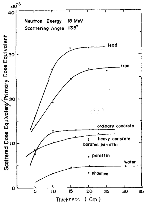
Fig. 14. Scattered dose equivalent ratios as a function of scatterer thickness for 18 MeV neutrons (scattering angle; 135^\circ )
