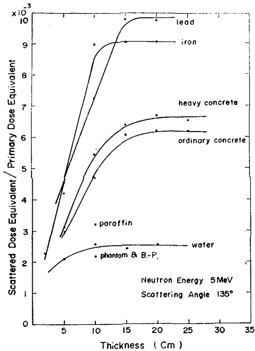
Fig. 12. Scattered dose equivalent ratios as a function of scatterer thickness for 5 MeV neutrons (scattering angle; 135^\circ )
