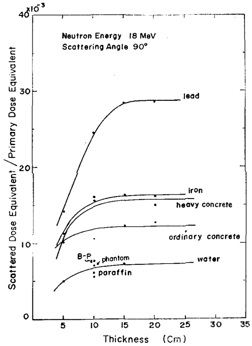
Fig. 13. Scattered dose equivalent ratios as a function of scatterer thickness for 18 MeV neutrons (scattering angle; 90^\circ )
