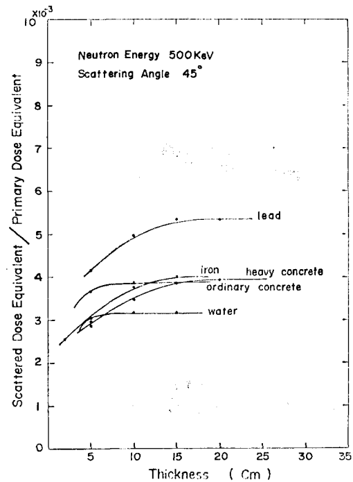
Fig. 3. Scattered dose equivalent ratios as a function of scatterer thickness for 500 keV neutrons (scattering angle; 45°)
