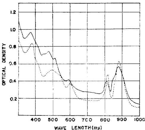
Fig. 1. In vivo absorption spectra of KS016 (---) and KS007(—), cells suspended in 60% sucrose solution.
