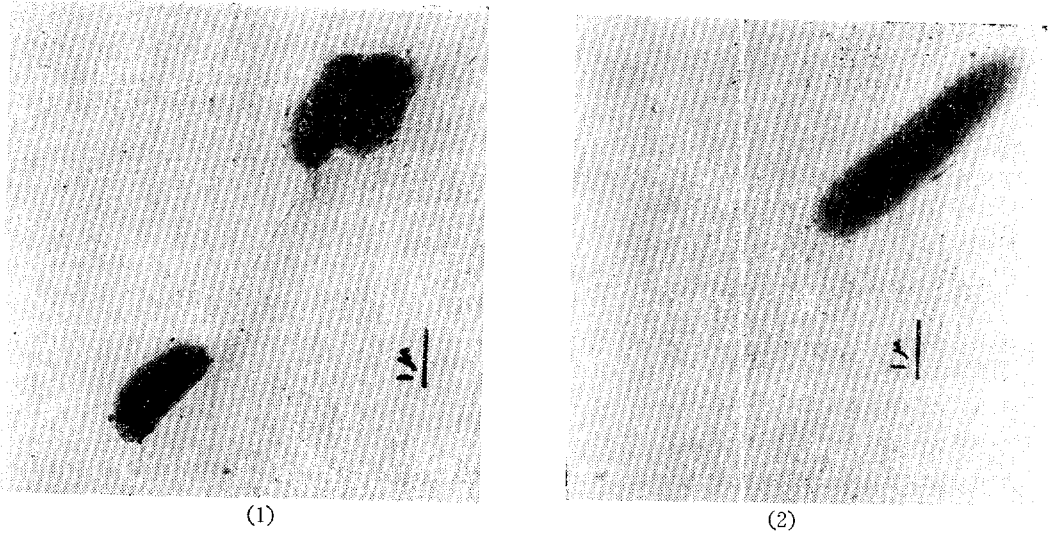
Plate 1. Electron micrographs of strain (1) KS016 and (2) KS007, magnification X8,000.
