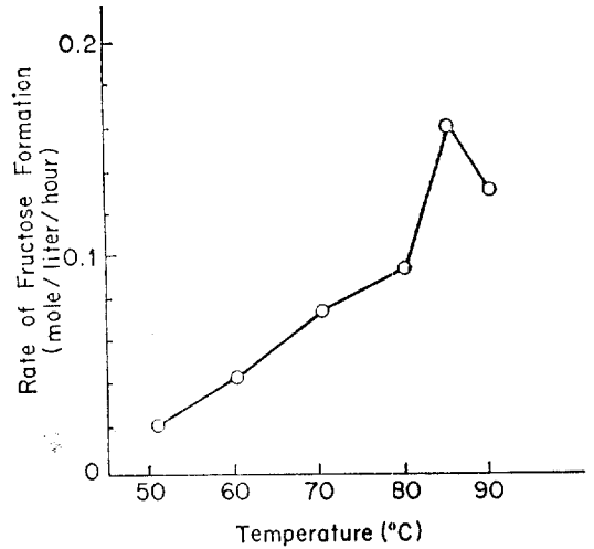
Fig. 5. Activation energy of the glucose isomerase reaction.
