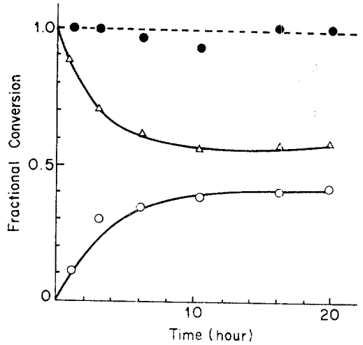
Fig. 9. Time course of glucose isomerization reaction by both the glucose determination and fructose determination. Fructose (○), glucose (△), total sugar (●).
