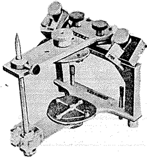
Fig. 1 Whip Mix Articulator
