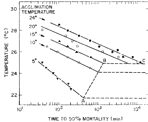
Fig. 3. Time to Death of a Representative Aquatic Organism (Chinook salmoe fry) as a Function of Exposure Temperature and Acclimation Temperature. At times beyond the lines A-B-C, there is indefinite survival.
