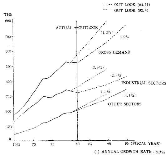
Fig. 1. Long-Term Electricity Demand Outlook
