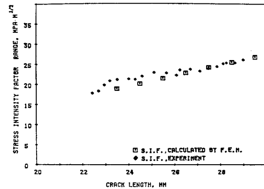
Fig. 14. Stress intensity factor range vs. crack length K-calculation of Brass + Hole (fatigue)
