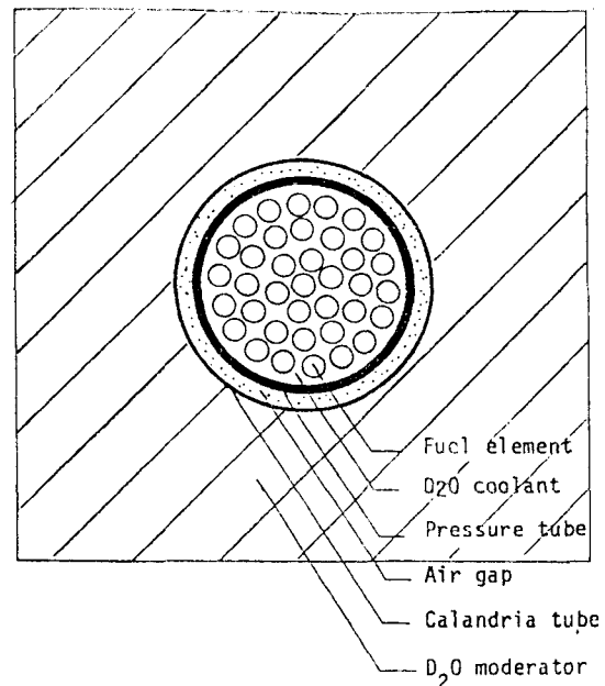
Fig. 1. Lattice Cell for 37 Elements Fuel
