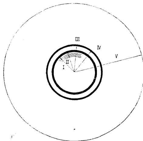
I. Fuel, Clad, Coolant annulus II. Pressure tube III. Air gap IV. Calandria tube V. Moderator
