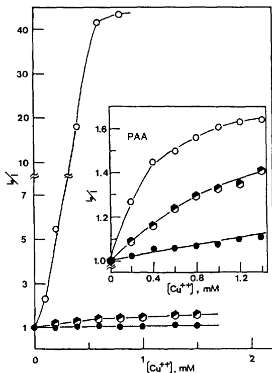
Figure 5. Stern-Volmer plots for quenching of \text{Ru}(\text{bpy})_3^{2+} luminescence by \text{Cu}^{2+} in 8 mM PMA and PAA(inset) solutions at pH 2( \bullet ), 5( \circ ), and 6.8( \square ).
