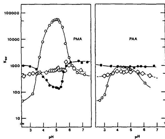
Figure 6. The pH dependences of K_{\text{SV}} 's for quenching reactions of \text{Ru}(\text{bpy})_3^{2+} with \text{Cu}^{2+} ( \circ ), nitrobenzene ( \bullet ) and \text{MV}^{2+} ( \diamond ) in 8 mM PMA(left) and PAA(right) solutions. Quencher concentration was fixed at 0.5 mM.
