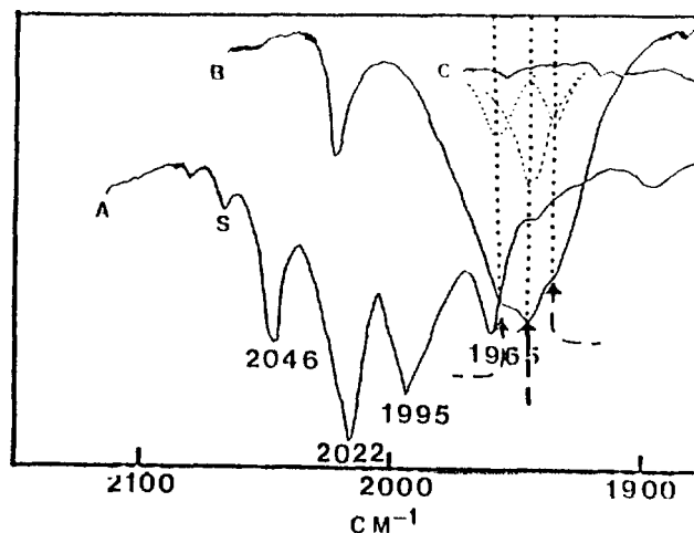
Figure 1. A. The \nu(\text{CO}) region of the infrared spectrum of \text{Fe}(\text{CO})_4(\text{Cp}_2\text{Zr}(\text{C}_8\text{H}_{17}))_2 in cyclohexane solution. B. The \nu(\text{CO}) region of the infrared spectrum of \text{Fe}(\text{CO})_4(\text{Cp}_2\text{Zr}(\text{CH}_3))_2 on a nujol mull. C. The \nu(\text{CO}) region of the infrared spectrum of \text{Na}_2\text{Fe}(\text{CO})_4 in THF solution.
