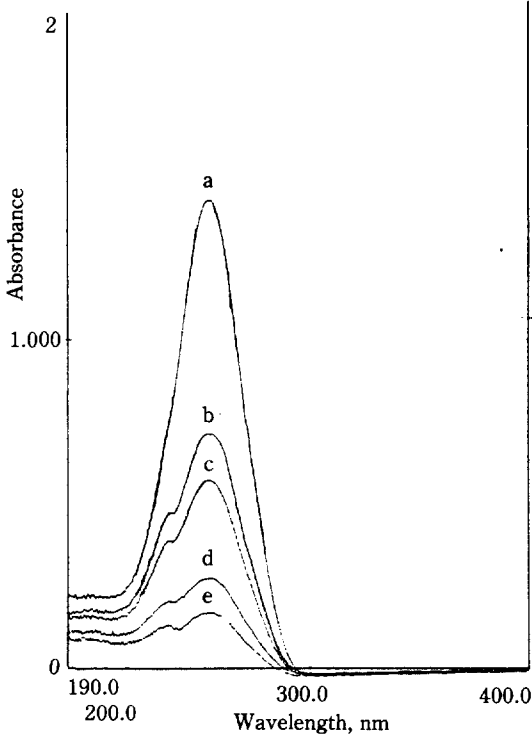
Fig. 2. UV-scanning spectra of 4-CB during biodegradation by the isolate DJ-12. a is the culture extracts at zero time and b, c, d and e are those of 6, 12, 18 and 24 hours old cultures, respectively.
