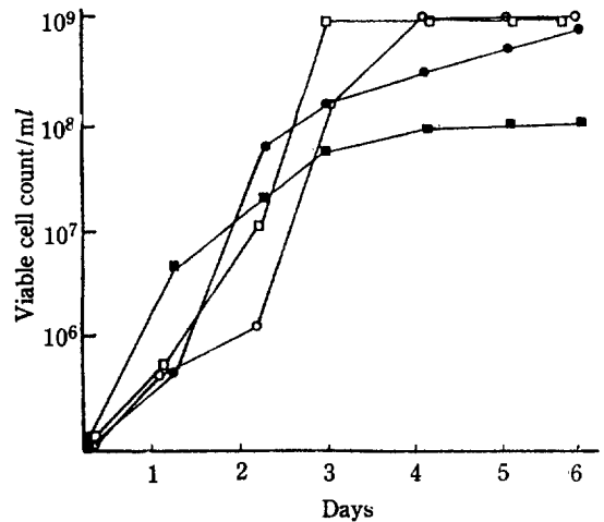
Fig. 1. Growth of the bacterial isolates on 4-CB or 2,4,5-T as a sole source of carbon in the MM2 liquid medium.
