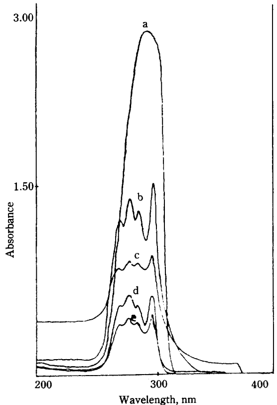
Fig. 3. UV-scanning spectra of 2, 4, 5-T during biodegradation by the isolate TP-1. a is the culture extracts at zero time and b, c, d, and e are those of 1, 2, 3, and 4 days old cultures, respectively.
