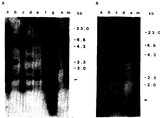
Fig. 1. Southern blot analyses of the exogenous DNAs from NIH3T3-subclones and from tumor tissues. The NIH3T3 subclones were established by transfection with the plasmid pKOneo and all tumors were induced by injection of these subclones into nude mice. Arrow indicates the presence of Hind III to Hind III fragment of neomycin resistant gene from the plasmid pKOneo. All DNAs were digested with Hind III endonuclease, fractionated on 0.7% agarose, blotted, and hybridized with the probe of pKOneo.
