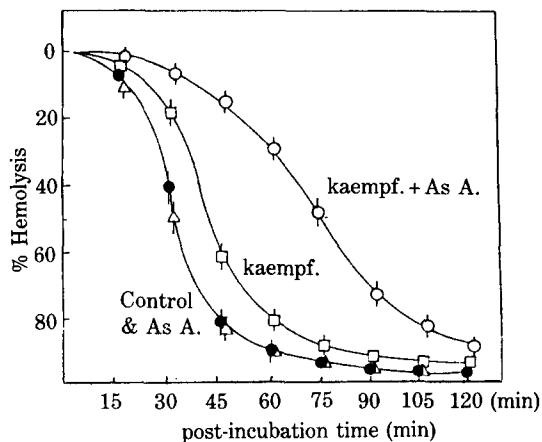
Fig. 4. Effects of kaempferol and L-ascorbic acid on the photosensitized hemolysis of rabbit erythrocytes (irradiation time = 20 min, sensitizer = rose-bengal).
