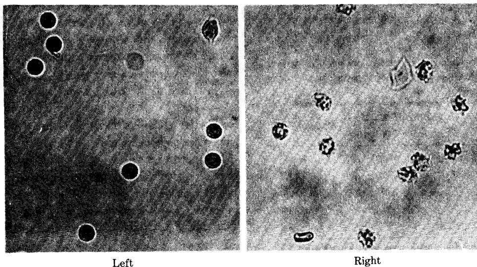
Fig. 6. Light microscopic pictures of rabbit erythrocytes treated 50 \mu M of quercetin (Left) and rutin (Right)
