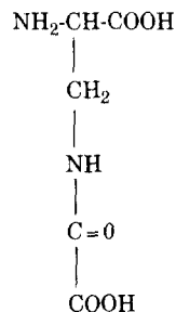
Fig. 2. Chemical structure of dencichine, \beta -N-oxalo-L- \alpha , \beta -diaminopropionic acid.
