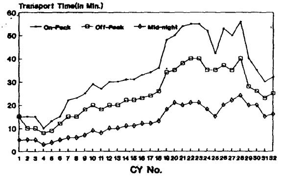
Fig. 4 Container Transport Times - Comparison of Container Transport Times (In-Field Data, 1990)
