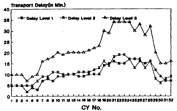
Fig. 5 Container Transport Delays - Comparison of Container Transport Delays (In-Field Data, 1990)
