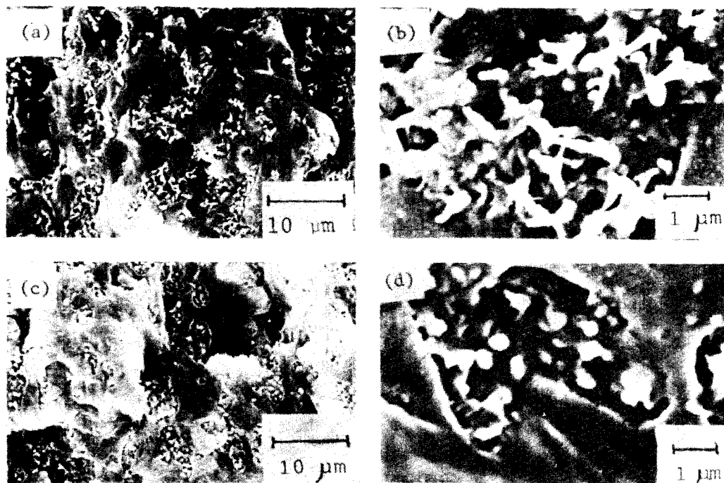
Fig. 10. SEM micrographs of the dynamically cured EPDM/PP/HDPE(ternary blends with DCP concentration of 0.67 phr ; the effect of the shear intensity. Mixer speed : (a) 20 rpm ( \times 2600 ); (b) 20 rpm ( \times 15,000 ) ; (c) 60 rpm ( \times 2600 ); (d) 60 rpm ( \times 15,000 ) (composition ; 25 : 56 : 19 EPDM : PP : HDPE)
