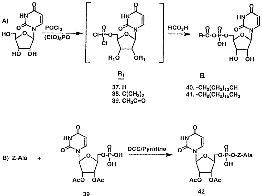
Scheme II
