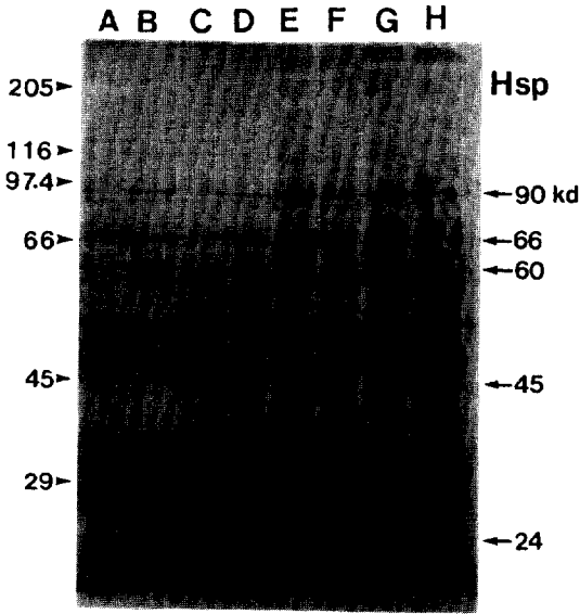
Fig. 2. Autoradiogram of the proteins synthesized in C. jejuni shocked with 1% and 3% ethanol. The cells were labeled with [ 35 S]-methionine in the medium without ethanol for 30 minutes after ethanol shock. Arrows on the left side are standard sizemarkers in kilodalton. Lanes: A, 42°C; B, 48°C (15 min); C, 1% (10 min); D, 1% (30 min); E, 1% (60 min); F, 3% (10 min); G, 3% (30 min); H, 3% (60 min).
