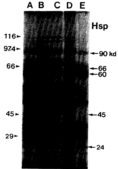
Fig. 3. Autoradiogram of the proteins synthesized in C. jejuni shocked with 5% ethanol. The cells were labeled with [ 35 S]-methionine in the medium without ethanol for 30 minutes after ethanol shock. Arrows on the left side are standard sizemarkers in kilodalton. Lanes: A, 5% (5 min); B, 5% (10 min); C, 5% (15 min); D, 42°C; E, 48 (15 min).
