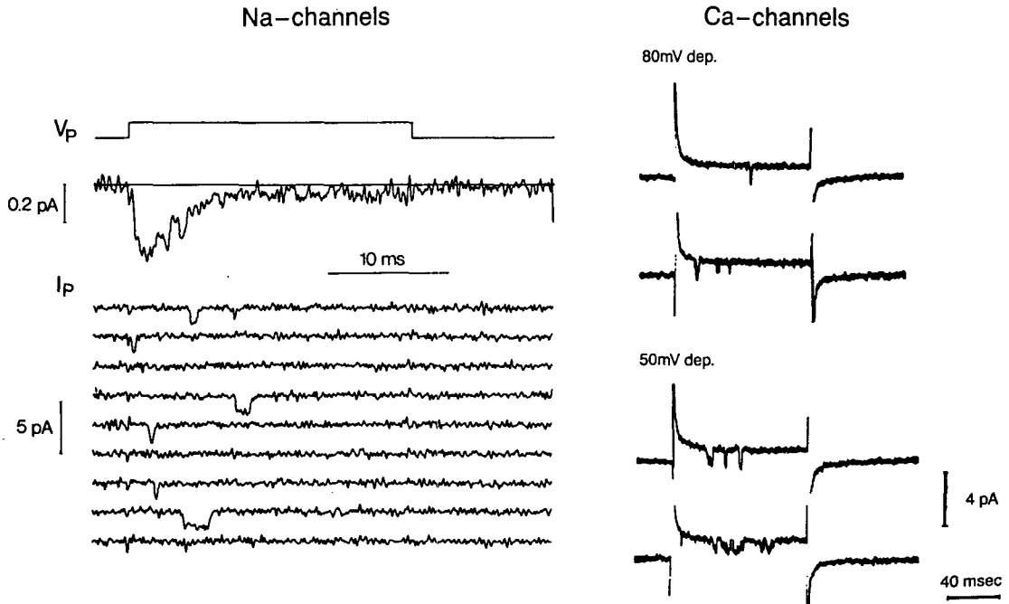
Fig. 3. Early records of voltage-activated single channels. The left side shows Na channels (adapted from Sigworth & Neher, 1980). The top trace is the voltage protocol. The second trace shows the average response from 300 voltage pulse depolarizations, and the following traces give examples of individual responses. It is seen that in some — but not in all — traces there are individual openings (downward deflection) of Na channels. The patch was hyperpolarized by 30 mV, and 40 mV depolarizing pulses are given.
