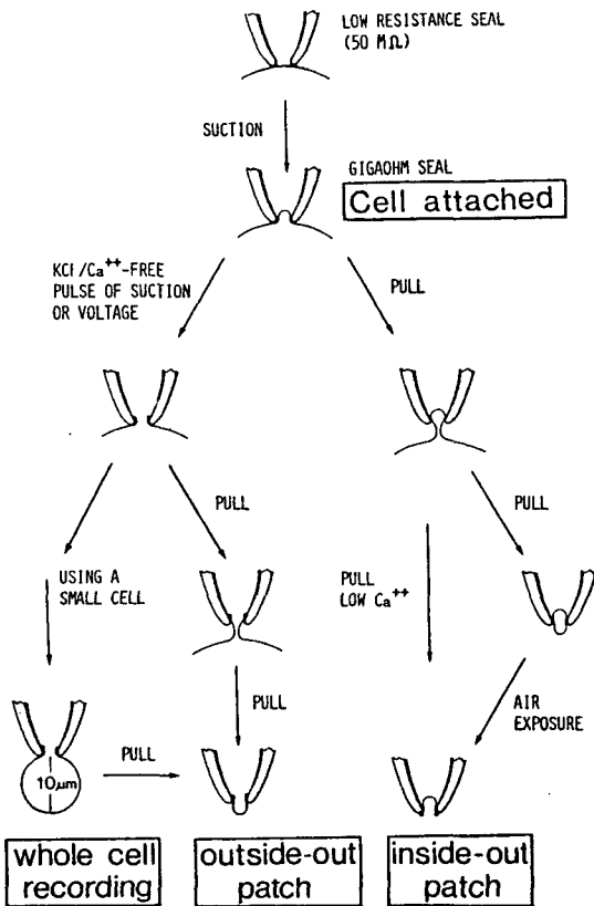
Fig. 4. Schematic representation of the procedures that lead to the different patch clamp configurations. From Hamill et al (1981).
