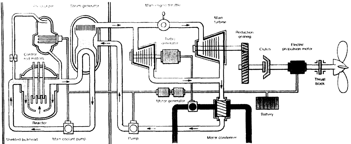
Pressurised-water nuclear propulsion system layout
