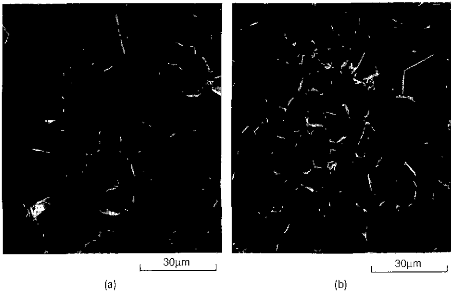
Fig. 10. Scanning electron micrographs of fracture surface of alumina under flexural test at 1200°C ; (a) compressive region, (b) tensile region.
