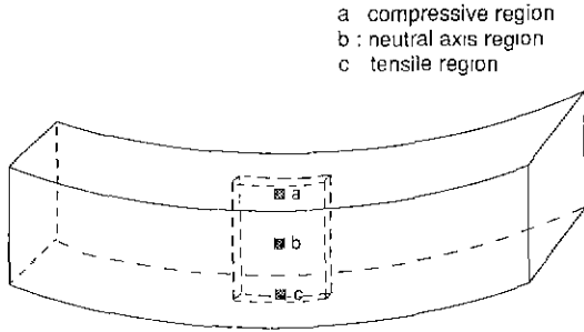
Fig. 6. A schematic drawing of a bending sample showing regions polished and etched for scanning electron microscopy.
