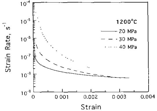
Fig. 3. Strain rate vs. strain of alumina under various flexural stresses at 1200°C.
