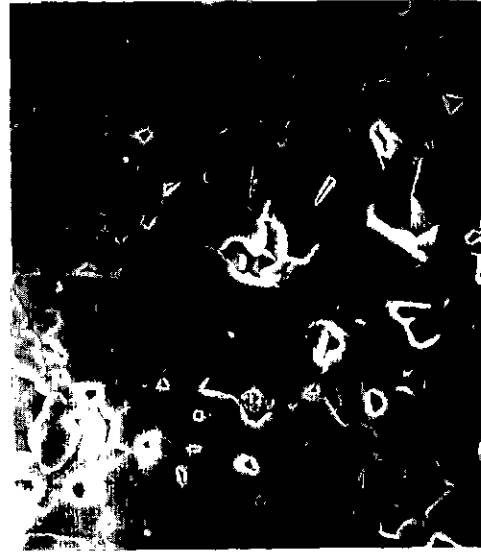
Fig. 7. Scanning electron micrograph of polished and etched cut section of alumina specimen without flexural stress.
