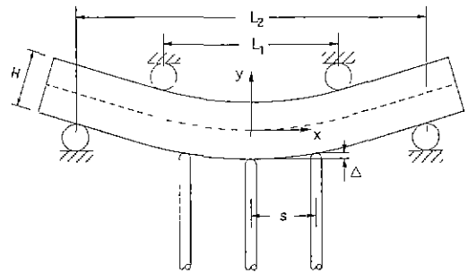
Fig. 1. A schematic drawing of 4-point bending creep test.
