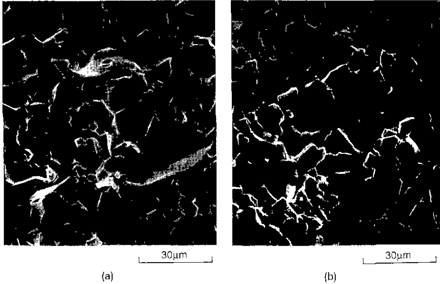
Fig. 11. Scanning electron micrographs of fracture surface of alumina under flexural stress of 30 MPa at 1200°C for 46 hours; (a) compressive region, (b) tensile region.
