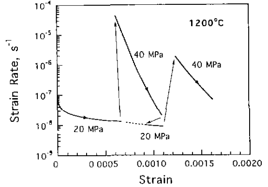
Fig. 5. Strain rate vs. cumulative strain of alumina under various loading paths at 1200°C.
