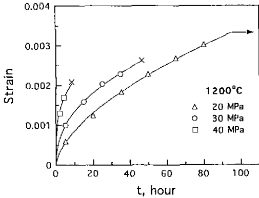
Fig. 2. Creep curves of alumina under various flexural stresses at 1200°C (× denotes the occurrence of fracture).
