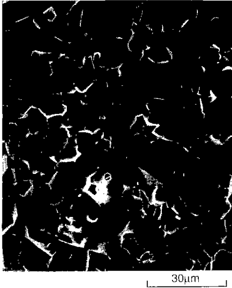
Fig. 9. Scanning electron micrograph of fracture surface of alumina under flexural test at room temperature.
