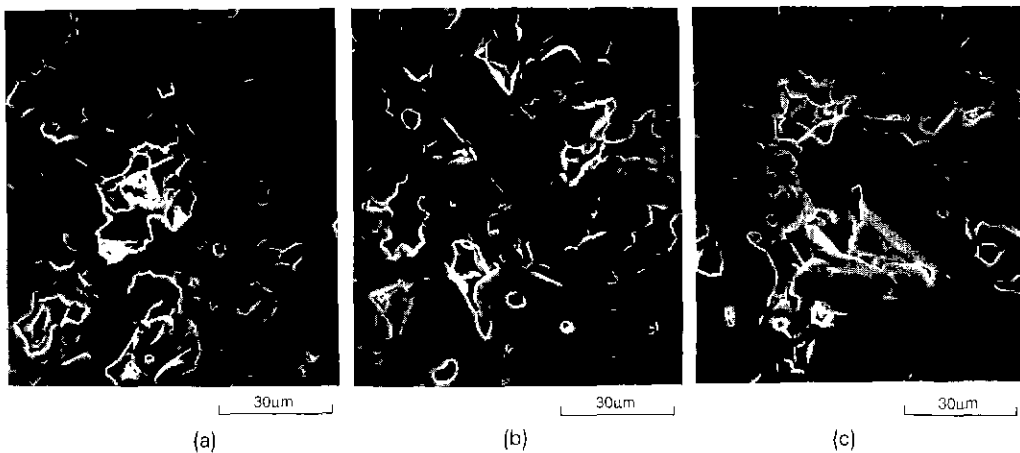
Fig. 8. Scanning electron micrographs of polished and etched cut section of alumina specimen under 20 MPa at 1200°C during 96 hours: (a) compressive region, (b) neutral axis region, (c) tensile region.
