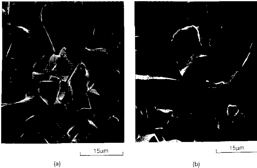
Fig. 12. Scanning electron micrographs of fracture surface for alumina crept under flexural stress of 30 MPa at 1200°C; (a) occurrence of fracture through the grain, (b) existence of pores in the fractured grain.
