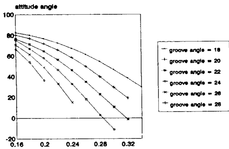
Fig. 9. Attitude angle for width ratio in case of eccentricity=0.1 and \Lambda=0.2
