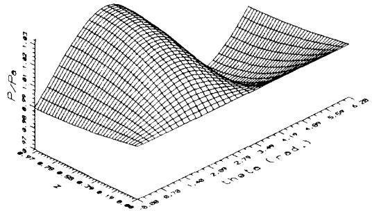
Fig. 7. The pressure distribution of plain journal bearing of \Lambda=0.2 and eccentricity=0.1 ( 0 \leq z \leq (L/R)/2 , 0 \leq \theta \leq 2\pi )
