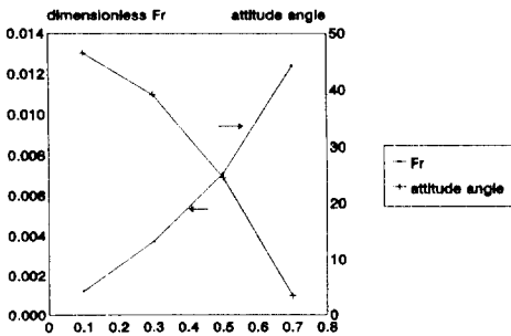
Fig. 10. Radial force and attitude angle for eccentricity in case of \Lambda=0.2 , width ratio=0.22, groove angle=24°
