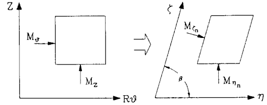
Fig. 4. Transformation of control volume
