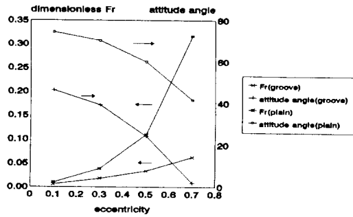
Fig. 13. Comparison of radial force and attitude angle for plain journal bearing and herringbone grooved journal bearing (width ratio=0.22, groove angle=24°) at \Lambda=1.0
