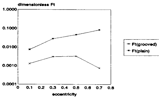
Fig. 14. Comparison of tangential force for plain journal bearing and herringbone grooved journal bearing (width ratio=0.22, groove angle=24°) at \Lambda=0.2
