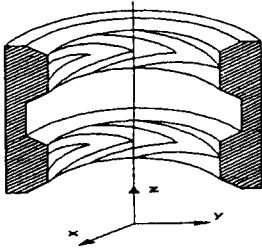
Fig. 2. Herringbone-grooved journal bearing
