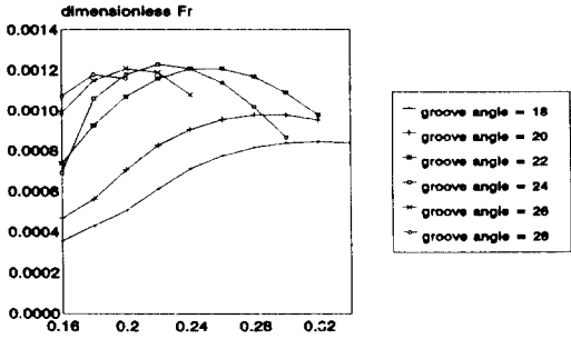
Fig. 8. Radial force for width ratio in case of eccentricity=0.1, \Lambda=0.2
