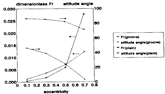
Fig. 12. Comparison of radial force and attitude angle for plain journal bearing and herringbone grooved journal bearing (width ratio=0.22, groove angle=24°) at \Lambda=0.2
