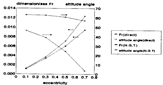
Fig. 18. Comparison of radial force and attitude angle for eccentricity by narrow groove theory and direct method at \Lambda=0.2 , width ratio=0.22 and groove angle=24°
