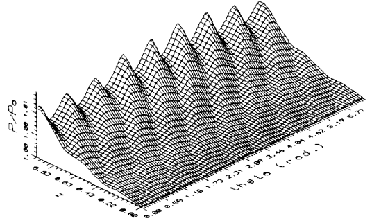
Fig. 6. The pressure distribution of herringbone-grooved journal bearing in case of groove numbers=8, \Lambda=0.2 , width ratio=0.32, groove angle= 24^\circ , and eccentricity=0.1 ( 0 \leq z \leq (L/R)/2 , 0 \leq \theta \leq 2\pi )
