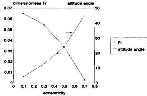
Fig. 11. Radial force and attitude angle for eccentricity in case of \Lambda=1.0 , width ratio=0.22 and groove angle=24°
