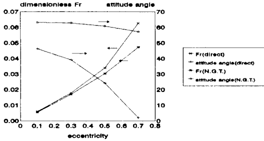
Fig. 19. Comparison of radial force and attitude angle for eccentricity by narrow groove theory and direct method at \Lambda=1.0 , width ratio=0.22 and groove angle=24°
