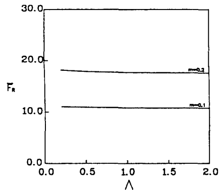
Fig. 13. Dimensionless friction force ( \omega_0 = 0.8 )
