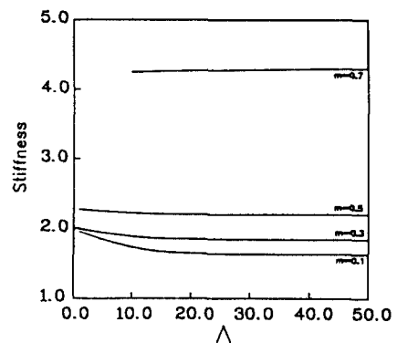
Fig. 14. Stiffness coefficient ( \bar{F}_{sr} = 0.3 )
