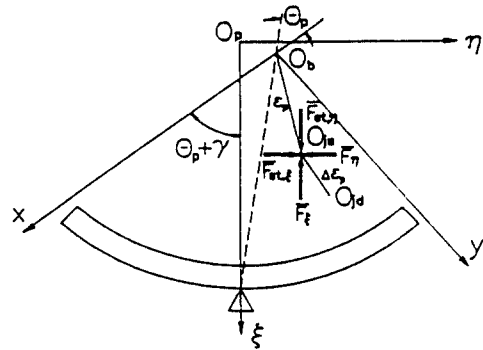
Fig. 4. Coordinate system for dynamic coefficients of fixed pad
