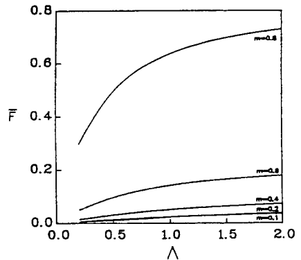
Fig. 8. Dimensionless load capacity ( \omega_e = 0.1 )
