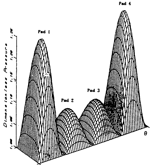
Fig. 7. Pressure distribution of tilting pad journal bearing
