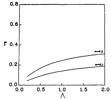
Fig. 12. Dimensionless load capacity ( \omega_0 = 0.8 )
