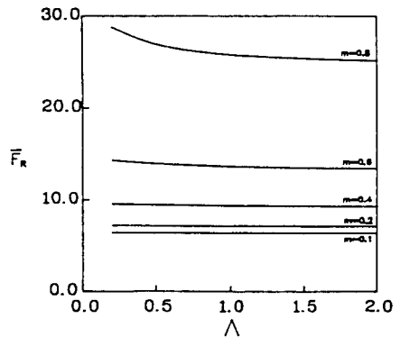
Fig. 9. Dimensionless friction force ( \omega_e = 0.1 )
