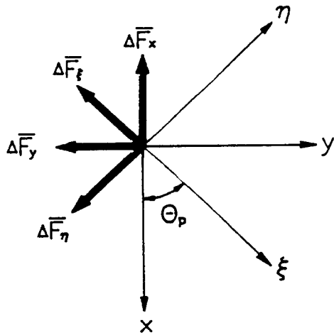
Fig. 6. Pad and bearing coordinate system for dynamic force and displacement
