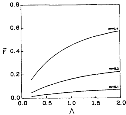
Fig. 10. Dimensionless load capacity ( \omega_0 = 0.5 )
