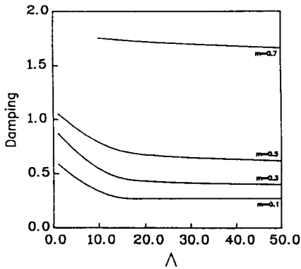
Fig. 15. Damping coefficient ( \bar{F}_r=0.3 )
