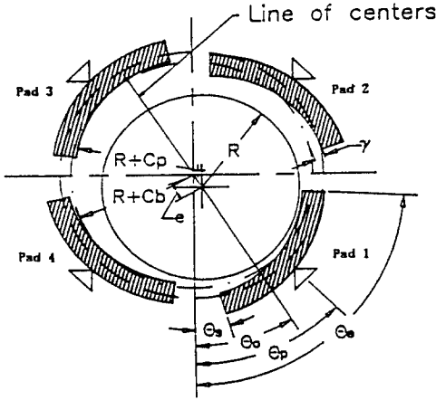
Fig. 1. Geometry of tilting pad journal bearing
