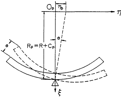
Fig. 5. Coordinate system for dynamic coefficients of tilting pad
