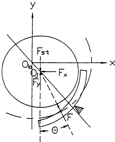
Fig. 3. Coordinate system of static forces
