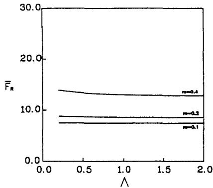
Fig. 11. Dimensionless friction force ( \omega_0 = 0.5 )
