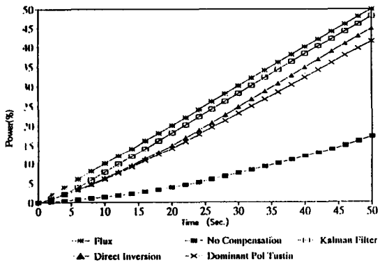
Fig. 3. Responses of 3 Digital Dynamic Compensation Methods of Rhodium SPND for Ramp Input and 2 Second Sampling Interval.
