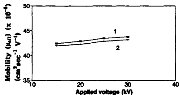
Figure 2. Effect of the applied voltage on the mobilities ( \mu_{\text{eff}} ). Phosphate buffer (30 mM, pH 7); other conditions were same as in Figure 1., 1. [\text{Pd}(\text{CN})_4]^{2-} , 2. [\text{Pt}(\text{CN})_4]^{2-} .
