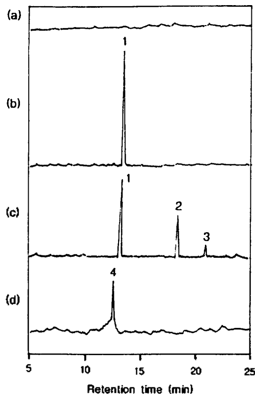
Figure 5. Electropherogram of chloro complexes of Pd and Pt. (a) [\text{PdCl}_6]^{2-} , [\text{PdCl}_5]^{2-} and [\text{PtCl}_6]^{2-} , (b) fresh solution of [\text{PtCl}_6]^{2-} , (c) aged solution of [\text{PtCl}_6]^{2-} (d) the solution (c) + 100 mM KCN.; other conditions were same as in Figure 1. Peaks: 1. [\text{PtCl}_6]^{2-} , 2 and 3. [\text{PtCl}_5(\text{OH})]^{2-} or [\text{PtCl}_5(\text{H}_2\text{O})]^{-} , 4. [\text{Pt}(\text{CN})_4]^{2-} .
