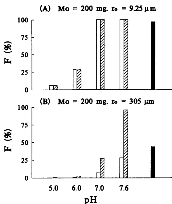
Fig. 8. Fraction dose absorbed ( F ) of benoxaprofen at various pH values. Dose is 200 mg and radii of particles are 9.25 \mu m (A) or 305 \mu m (B). The fractions dose absorbed are estimated using I_s=0 or 1 and An=7 . The closed bars represent the reported values in the literature (Wolen et al. , 1979).
