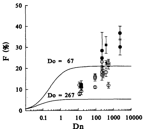
Fig. 6. Fraction dose absorbed ( F ) of griseofulvin. Predicted values are shown by solid lines. Values of parameters used for calculations: Do=67 and 267 , An=7 , Is=0 . Human data were taken from Atkinson et al. (1962), Khalafalla et al. (1980), and Terhaag et al. (1985). ○: Atkinson et al. (1962)-tablets, ●: Atkinson et al. (1962)-capsules, ▲: Khalafalla et al. (1980), ■: Terhaag et al. (1985)
