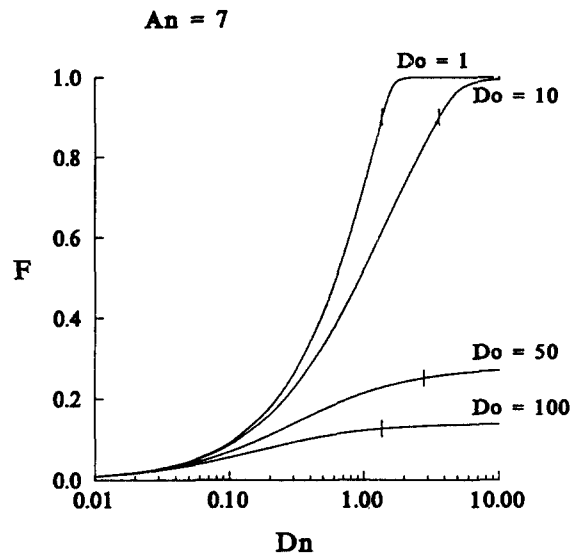
Fig. 3. Plot of fraction dose absorbed ( F ) versus dissolution number ( Dn ) at several different dose numbers ( Do=1, 10, 50, 100 ). Bar(l) indicates 90% of maximal F which can be obtained at no dissolution limitation. Values of parameters used for calculations: An=7, Is=0 .
