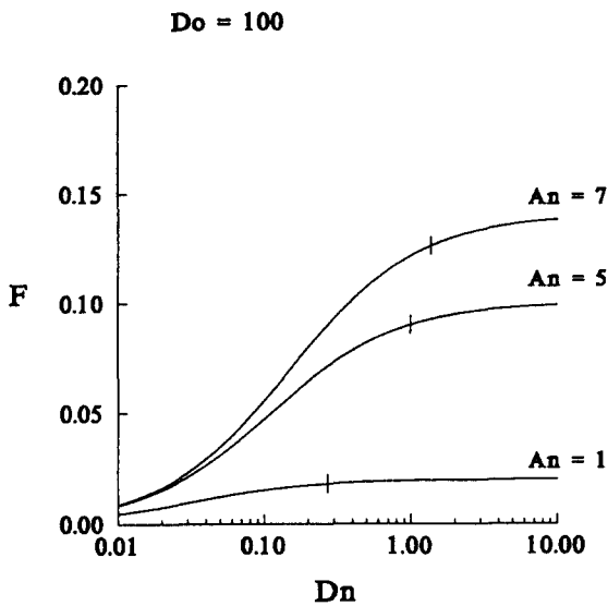
Fig. 2. Plot of fraction dose absorbed ( F ) versus dissolution number ( Dn ) at several different absorption numbers ( An=1, 5, 7 ). Bar(l) indicates 90% of maximal F which can be obtained at no dissolution limitation. Values of parameters used for calculations: Do=100, Is=0 .
