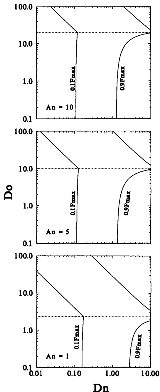
Fig. 4. Ten percent ( 0.1 \cdot F_{max} ) and 90% ( 0.9 \cdot F_{max} ) of maximal F (at no dissolution limitation; Dn \rightarrow \infty ) in the plot of Do versus Dn for An of 1, 5, and 10. Dotted lines represent the dose numbers at Dn \rightarrow \infty .
