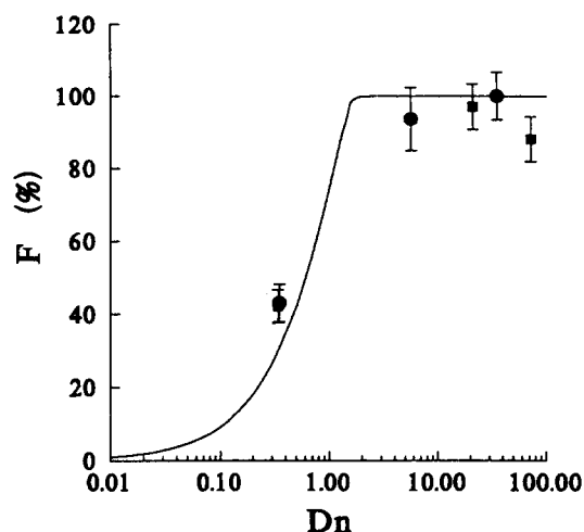
Fig. 5. Fraction dose absorbed ( F ) of digoxin. Predicted values are shown by a solid line. Values of parameters used for calculations: Do=0.1 , An=7 , Is=0 . Human data were taken from Jounela et al. (1975) and Johnson et al. (1978).
