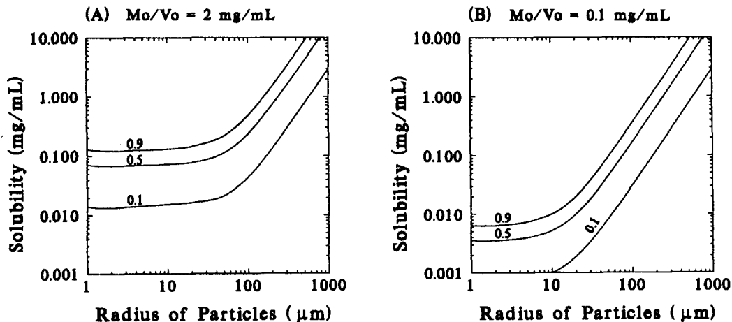
Fig. 7. Contours of fraction dose absorbed ( F ) in the plot of solubility and radius of particles for M_o/V_o=2 mg/mL (A) or 0.1 mg/mL (B). Values of parameters used for calculations: An=7 , Is=0 .
