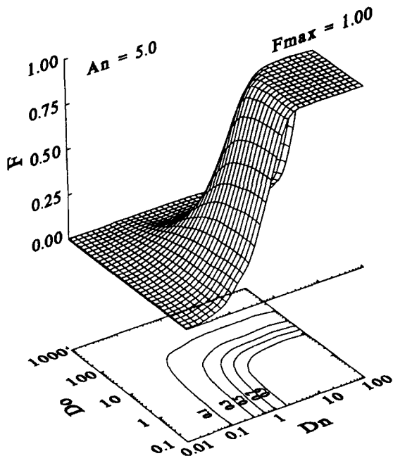
Fig. 1. Three dimensional graph and contour of the fraction dose absorbed ( F ) in the plot of dose number ( Do ) versus dissolution number ( Dn ) at An=5 and Is=0 .
