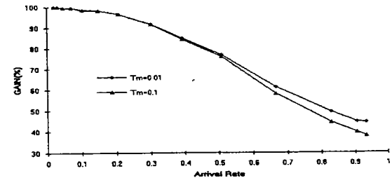
(Fig. 8) Gain of mean number of messages per job over the bidding algorithm
