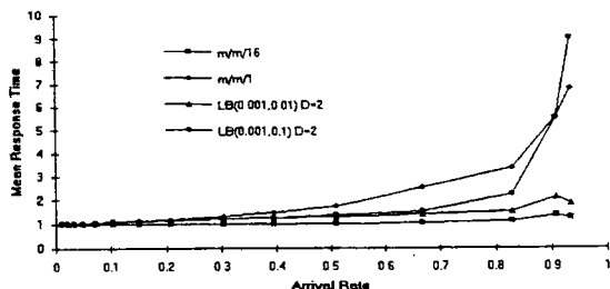
(Fig. 1) Comparison of mean response time vs. arrival rate( n=16 )
