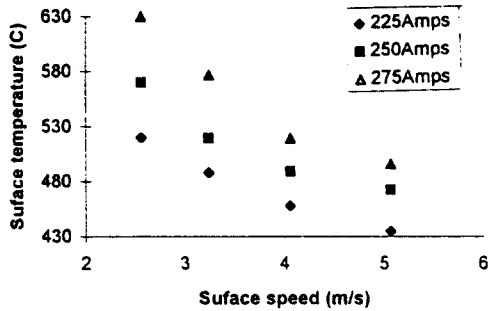
Fig. 7 Surface temperature versus surface velocity at variable plasma current(77.5mm diameter workpieces, 0.124mm/rev feed)
