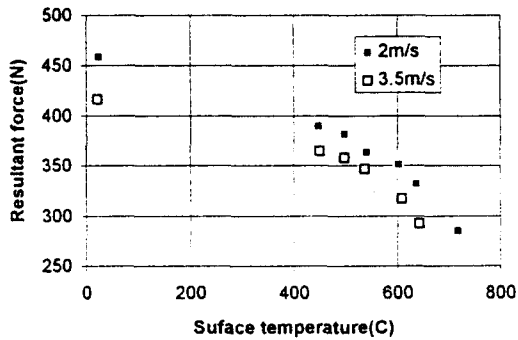
Fig. 13 Resultant cutting force versus surface temperature (0.124mm/rev, cutting speed 3.5m/s and 2m/s)
