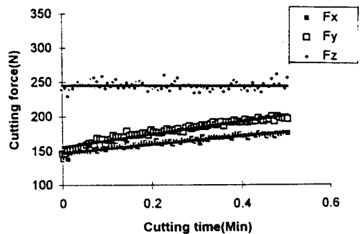
Fig. 11 Components of cutting force as a function of cutting time during PHM(plasma current 250Amp, cutting speed 6.28m/s, 0.124mm/rev feed)
