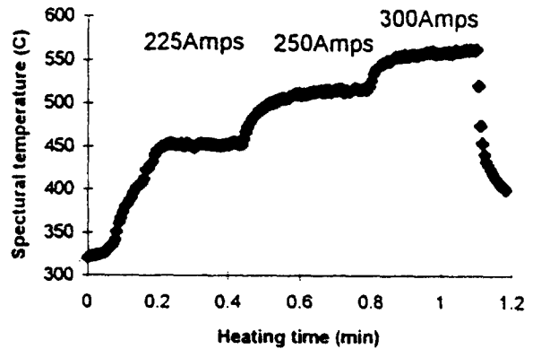
Fig. 4 Spectral temperature as function of heating time (82mm diameter workpiece, 0.124mm/rev feed, 800rpm)
