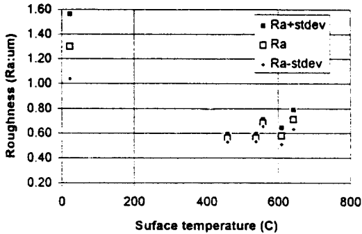
Fig. 15 Surface roughness versus surface temperature(cutting speed 3/5m/s, feed 0.124mm/rev, cutting time 0.5min)
