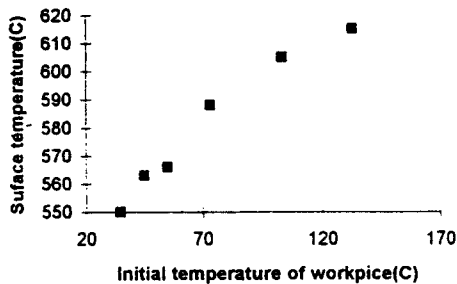
Fig. 9 Surface temperature versus workpiece initial temperature(3.64m/s surface speed, 66.2mm diameter workpiece, 0.124mm/rev feed)
