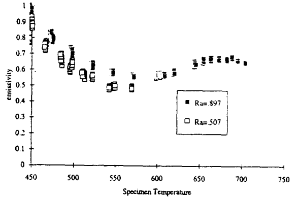
Fig. 3 Emissivity for two different Raroughness values
