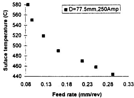
Fig. 8 Surface temperature versus feed rate(3.24m/s surface velocity, 250Amp plasma current, 77.5mm diameter workpiece)
