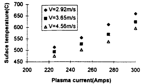
Fig. 6 Surface temperature versus plasma current at variables surface speed(69.0mm diameter workpieces, 0.124mm/rev feed)
