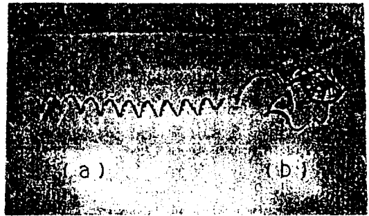
Fig. 14 Comparison of formed chip a) Conventional cutting b) PHM
