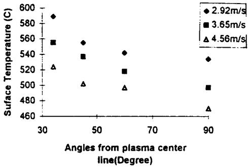
Fig. 5 Surface temperature versus variable angles from plasma centerline(250 Amp plasma current, 69.7mm diameter workpieces, 0.124mm/rev feed)
