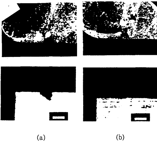
Fig. 12 Photograph of the tool wear(cutting speed 5.5m/s, feed 0.124mm/rev, cutting length 50mm, depth of cut 1.5mm)
