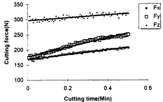
Fig. 10 Components of cutting force as a function of cutting time during conventional machining(cutting speed 6.28m/s, 0.124mm/rev feed)
