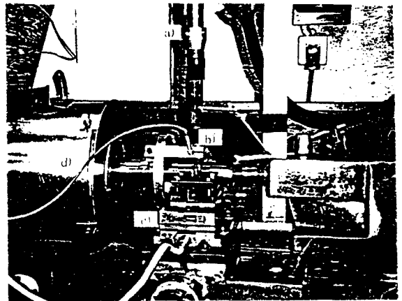
Fig. 1 Photograph of plasma hot machining equipment
