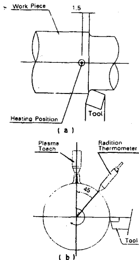
Fig. 2 Set up plasma heating a) Schematic diagram of plasma arc torch b) Set up for temperature measurement
