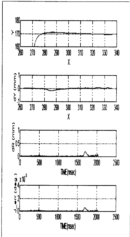
Fig. 10 The experimental results for position trajectory trajectory tracking of point ① at Cartesian Space with 2 kg payload
