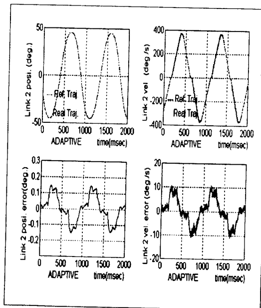
Fig. 6 The experimental result for position and velocity trajectory tracking of joint 2 with payload(2.0kg)
