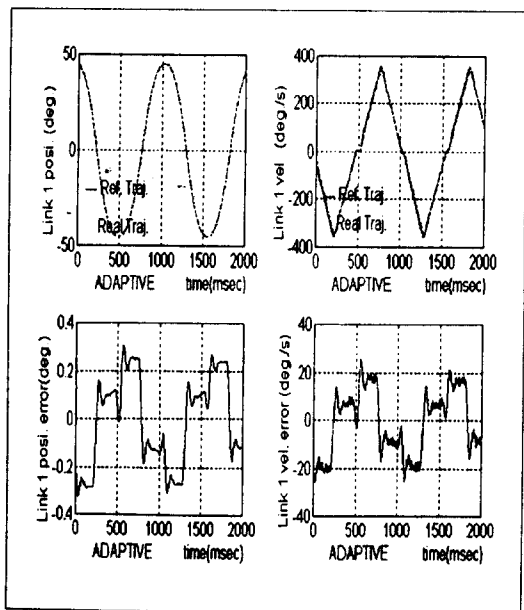
Fig. 5 The experimental result for position and velocity trajectory tracking of joint 1 with payload(2.0kg).
