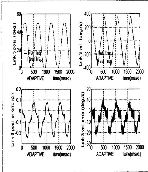
Fig. 7 The experimental result for position and velocity trajectory tracking of joint 3 with payload(2.0kg)
