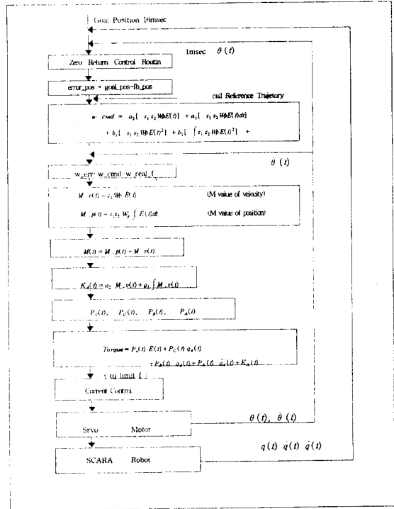
Fig. 4. Flow chart of adaptive control using TMS320C3x assembler.
