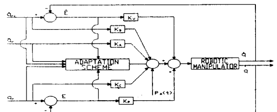
Fig. 1 The block diagram of model reference adaptive control for robot manipulator.
