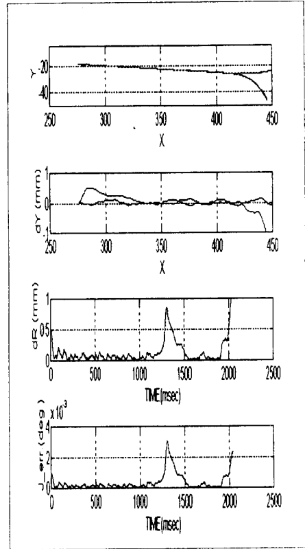
Fig. 13 The experimental results of PID controller for position trajectory tracking of point ② at Cartesian Space with 2 kg payload.
