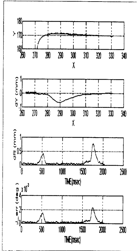
Fig. 11 The experimental results of PID controller for position trajectory tracking of point ① at Cartesian space with 2 kg payload.
