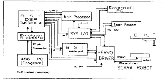
Fig. 2. The block diagram of control system.
