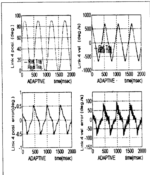
Fig. 8 The experimental result for position and velocity trajectory tracking of joint 4 with payload(2.0kg)
