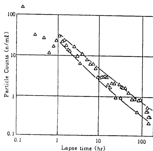
Fig. 9. Transition of particle counts(Outside pressure type UF).
