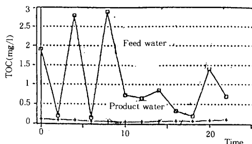
Fig. 17. Example of TOC treatment by biodegradation.
