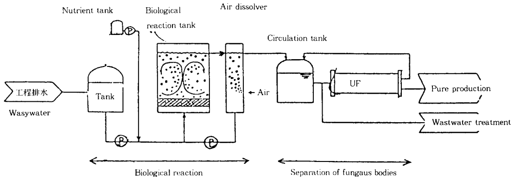
Fig. 15. Example of biological decomposing system(trade name: Biofilter & Preblock).
