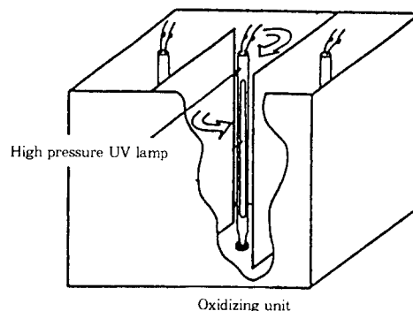
Fig. 13. High pressure ultraviolet ray oxidizing equipment.
