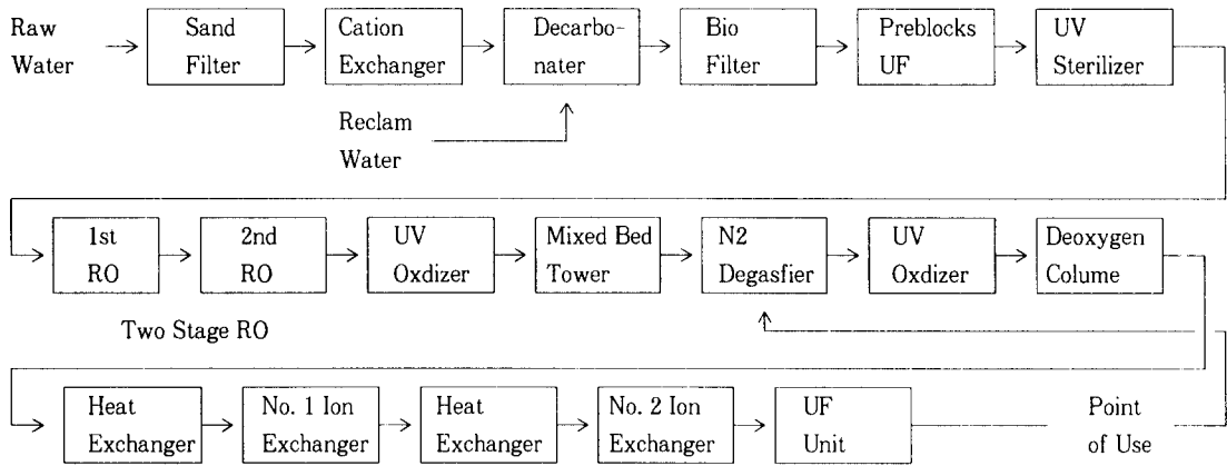
Fig. 1. Example of ultrapure water production system.
