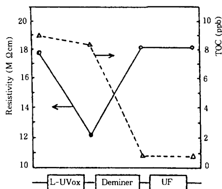
Fig. 12. Example of change in water quality in the secondary pure water production system.
