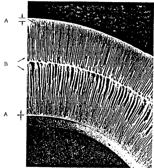
Fig. 6. Section of capillary UF (by SEM).
