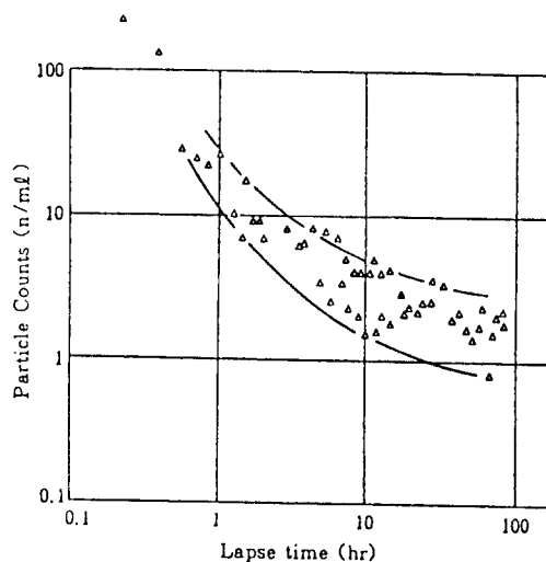
Fig. 8. Transition of particle counts(Inside pressure type UF).
