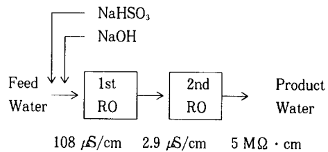
Fig. 4. Operation data of two stage RO.
