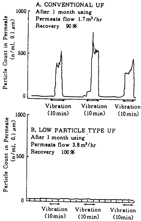
Fig. 10. Particle generation from UF element with vibration.
