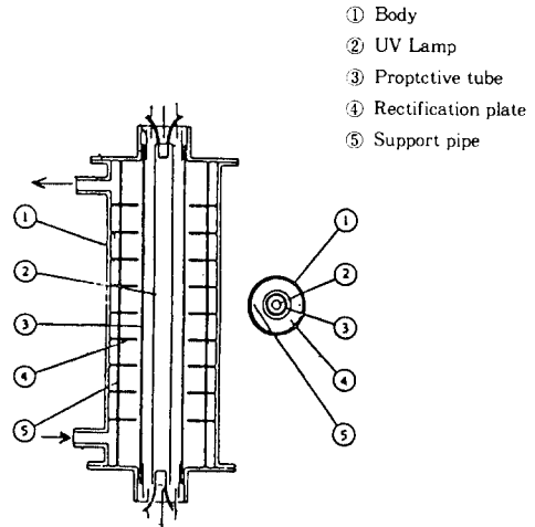
Fig. 11. Example of low pressure ultraviolet ray oxidizing equipment.
