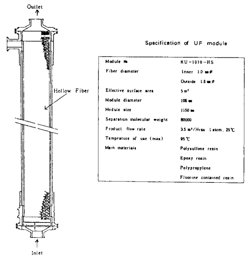
Fig. 7. Structure of capillary UF module.
