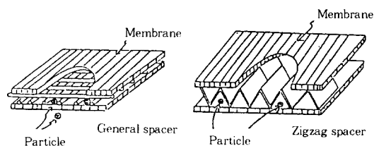
Fig. 16. UF module developed for removing fungus bodies (trade name: Preblocks).
