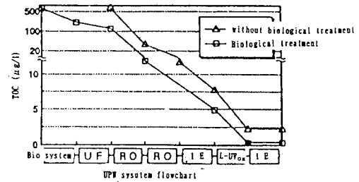
Fig. 18. Example of TOC behavior within the ultra-pure water system.
