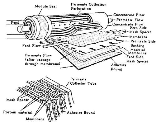
Fig. 3. Structure of spiral RO element.
