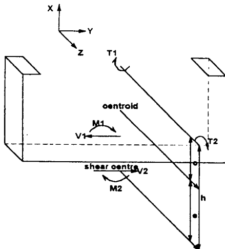
Fig. 1 Coordinates and stress resultant
