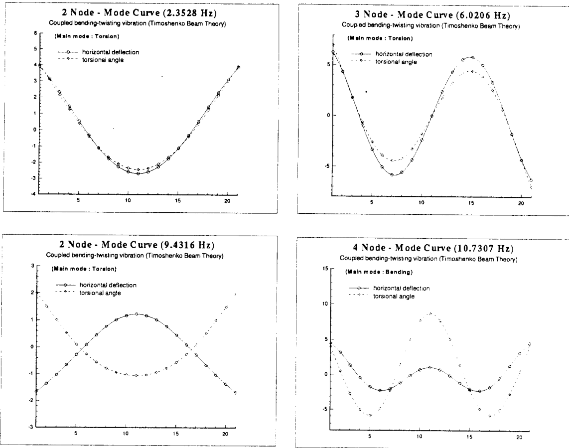
Fig. 10 Mode curves for a channel-type uniform beam
