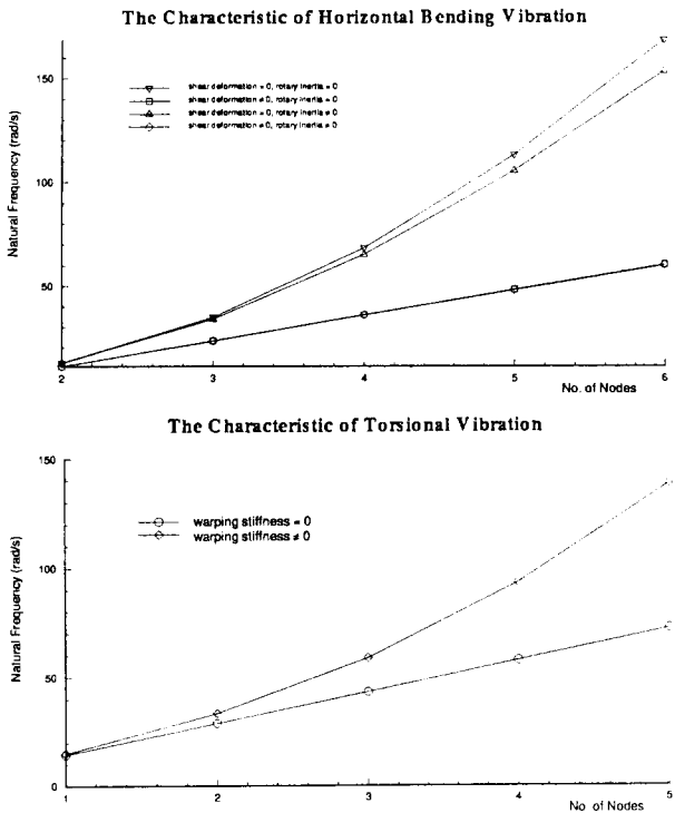
Fig. 8 Parametric analysis for the bending and torsional analysis
