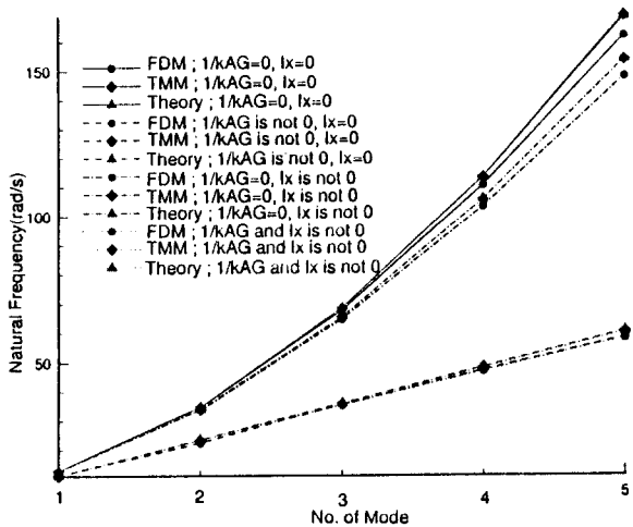
Fig. 5 Natural frequencies for coupled bending and twisting vibration with warping stiffness(rad/sec)
