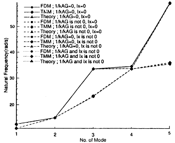
Fig. 2 Natural frequencies for uncoupled horizontal vibration(rad/sec)
