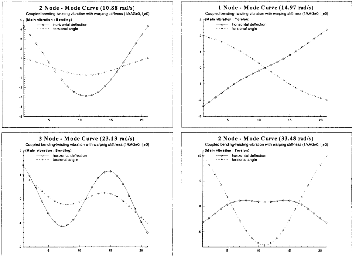
Fig. 9 Mode curves for a box-like uniform beam
