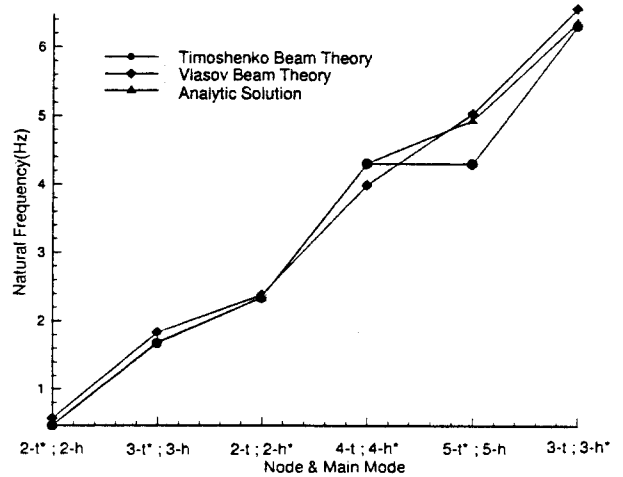
Fig. 7 Coupled bending-torsional vibration for a nonuniform beam(t: torsional mode, h: horizontal bending mode, *: main mode)
