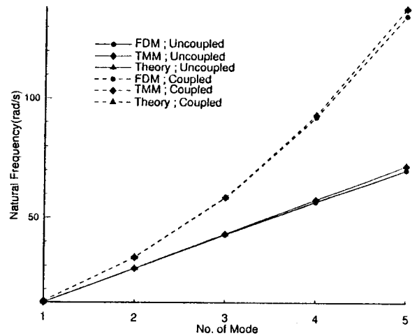
Fig. 3 Natural frequencies for uncoupled torsional vibration(rad/sec)
