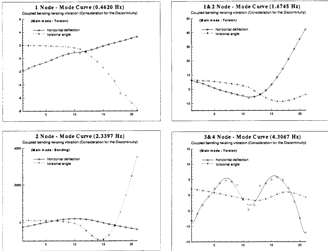
Fig. 11 Mode curves for a non-uniform beam
