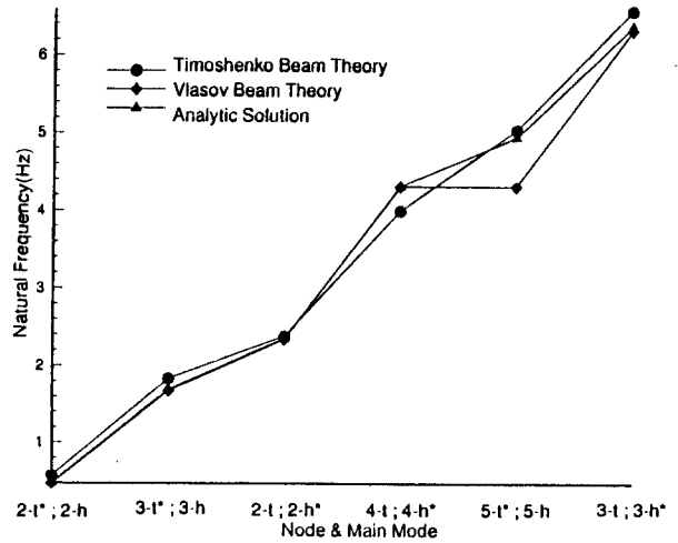
Fig. 6 Coupled bending-torsional vibration for a channel type uniform beam(t: torsional mode, h: horizontal bending mode, *: main mode)
