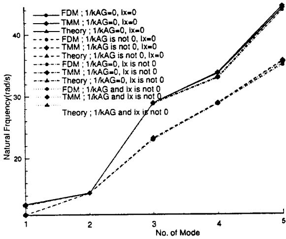
Fig. 4 Natural frequencies for coupled bending and twisting vibration with zero warping stiffness(rad/sec)
