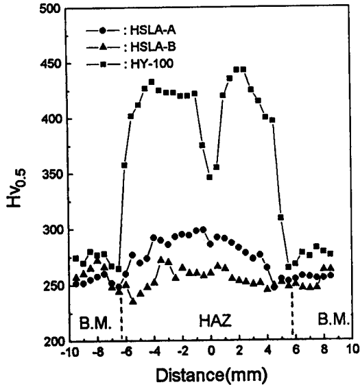
Fig. 5 Hardness distribution in GMA welded joint of HSLA-A, HSLA-B and HY-100 steels.
