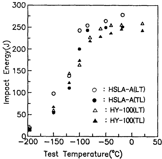
Fig. 4 Variations of impact energies with test temperature in LT and TL direction of 650°C aged HSLA-A and 660°C aged HY-100 steels.
