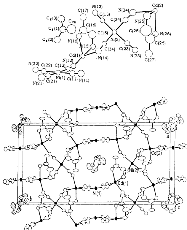
Figure 1. Structure of Cd(NH 2 CH(CH 3 )CH 2 NH 2 )Ni(CN) 4 ·0.25 p -(CH 3 ) 2 C 6 H 4 . Top: Asymmetric unit with atomic notations; bottom: projection along the c -axis. The Cd and Ni atoms are shown as solid ellipsoids and the guest atoms are dotted.
