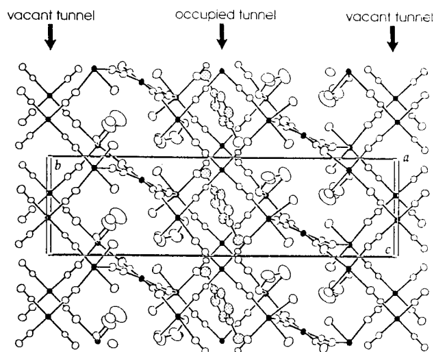
Figure 2. Structure of Cd(NH 2 CH(CH 3 )CH 2 NH 2 )Ni(CN) 4 ·0.25 p -(CH 3 ) 2 C 6 H 4 along the a -axis in the range of ca. 0.7 a , 1.2 b and 3 c . The Cd and Ni atoms are shown as solid ellipsoids and the guest atoms are dotted.
