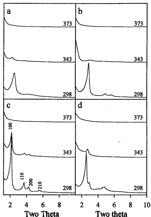
Figure 1. XRD patterns of mesoporous materials: (a) SiMCM-41A; (b) SiMCM-41B; (c) SiMCM-41C; (d) MCM-48. The XRD patterns were obtained with Cu K\alpha X-ray source using Rigaku D/MAX-III (3 kW) instrument, after the samples were heated in distilled water for 12 h. Numbers denote the heating temperatures in kelvin.
