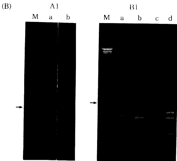
Fig. 4. The 3rd RFLP analysis of the 16S rDNA clones belonging to subgroup A1 and B1 by AluI restriction. The RFLP types were classified(A) according to their mobility patterns in 3% agarose gel(B). \lambda / HindIII marker was run on the parallel lanes(M) and arrows indicate the mobility of 0.56 kb marker DNA.
