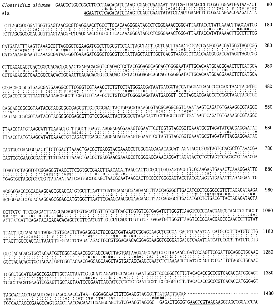
Fig. 6. Alignment of 16S rDNA sequences of the A1a-K2 clone and Clostridium ultunae . Differences between these sequences are indicated by asterisks(*). PCR primer sequences are underlined.
