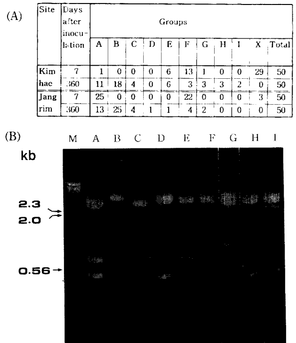
Fig. 2. The 1st RFLP analysis of 16S rDNA clones by SacII + EcoRI restriction. The RFLP types were classified and counted(A) according to their mobility patterns in 2% agarose gel(B). \lambda - HindIII marker is shown(lane M).
