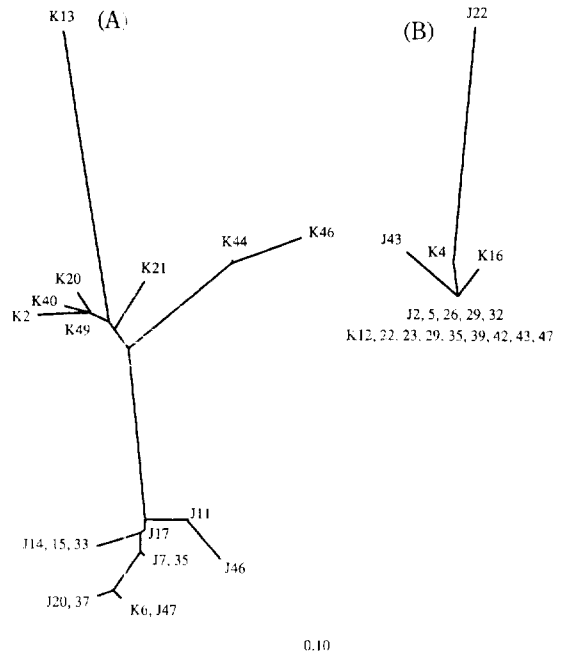
Fig. 5. Phylogenetic radiograms showing the divergence of the 16S rDNA clones belonging to A1a(A) and B1d(B) groups, respectively. Scale bar represents 0.1 substitutions per nucleotide position.
