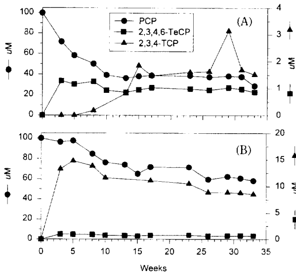
Fig. 1. Anaerobic degradation of PCP and its byproducts by the anaerobic sludge from Jangrim sewage treatment plant(A) and the leachate from Kimhae landfill site(B).
