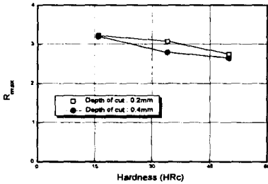
Fig. 3 Surface roughness(Rmax) vs. Hardnesses of workpiece for STD11
