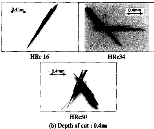
Fig. 9 Chips of STD11 for various hardnesses
