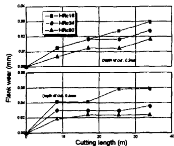
Fig. 2 Flank wear vs. Cutting length for STD11
