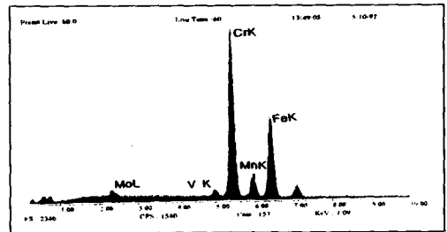
Fig. 8 EDX analysis of the Cr, Fe carbide in the HRc16 workpiece
