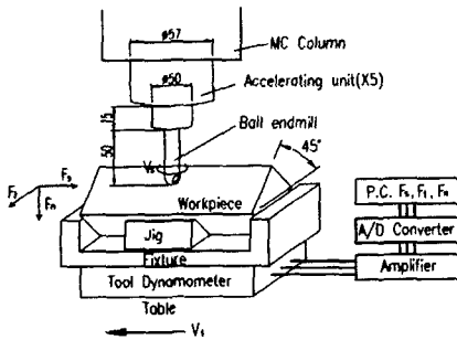
Fig. 1 Experimental system
