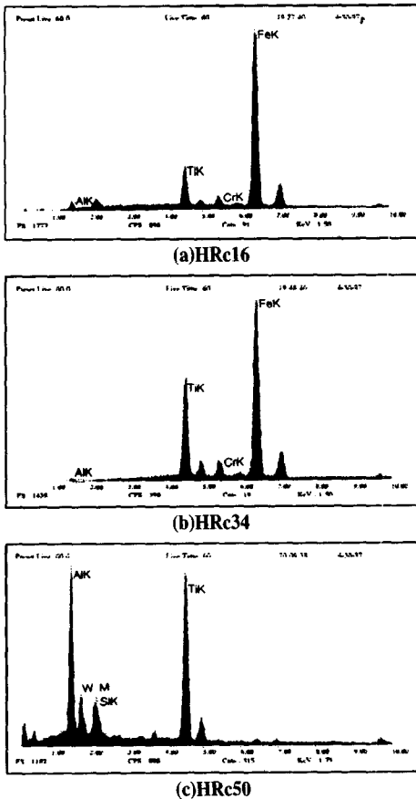
Fig. 6 EDX analysis of CBN ball endmill (Depth of cut : 0.4mm)
