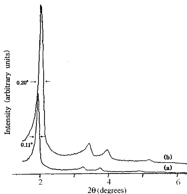
Figure 8. XRD patterns of (a) as-made and (b) calcined MCM-41 synthesized from a gel of \text{SiO}_2 :0.27CTABr:0.19TMAOH:40H 2 O aged 24 h and reacted at 150 °C for 48 h. Degrees in figure indicate the full width at half maximum of (100) peak.
