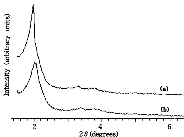
Figure 1. XRD patterns of MCM-41 synthesized from a gel of \text{SiO}_2 : 0.27CTACl: 0.18TMAOH: 30H 2 O using different silica source: (a) Sigma fumed silica and (b) Cab-O-Sil fumed silica.
