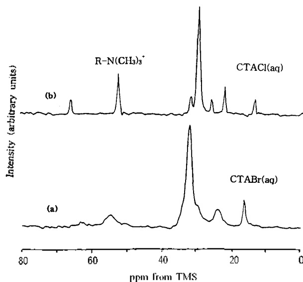
Figure 9. 13 C MAS NMR spectra with high-power proton decoupling of 7% aqueous solutions of (a) CTABr and (b) CTACl.
