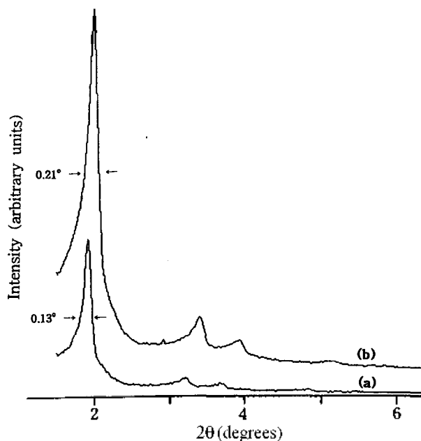
Figure 7. XRD patterns of (a) as-made and (b) calcined MCM-41 synthesized from a gel of \text{SiO}_2 :0.20CTACl:0.18TMAOH:25H 2 O aged for 24 h and reacted at 150 °C for 48 h. Degrees in Figure indicate the full width at half maximum of (100) peak.
